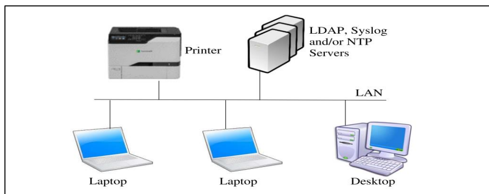
Figure 1: TOE Architecture
